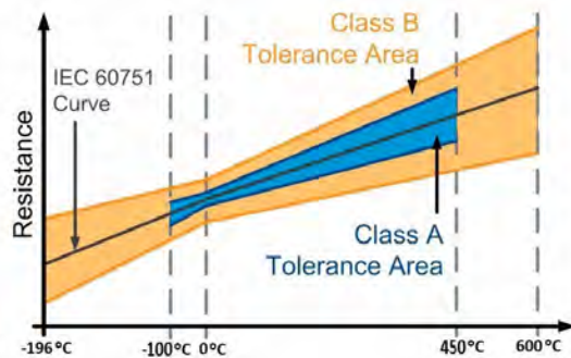
Figure 8: Sensor Accuracy Curve
