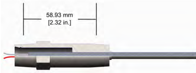
Figure 14: Dimensions
