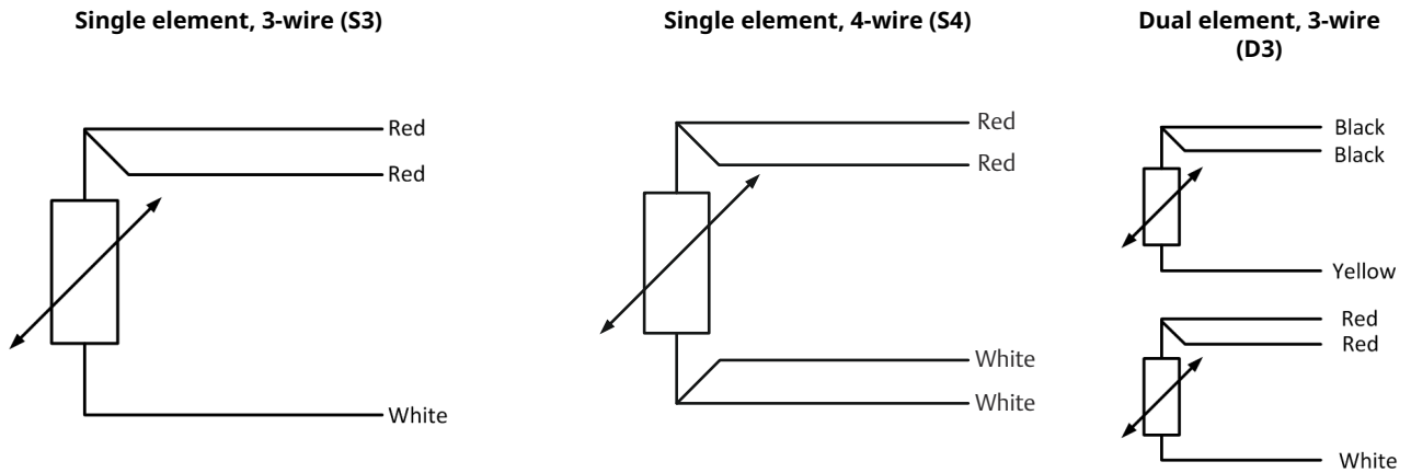
Figure 9: RTD Lead Wire Configurations
