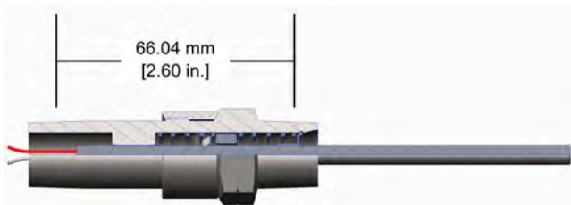
Figure 13: Dimensions
